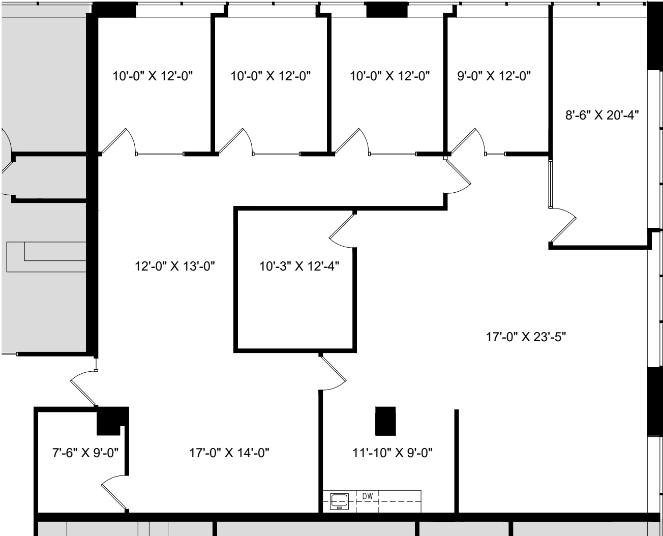
SUITE 120 - 2,679 RSF NOT TO SCALE
